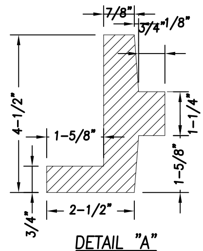
BOLT DOWN DETAIL
