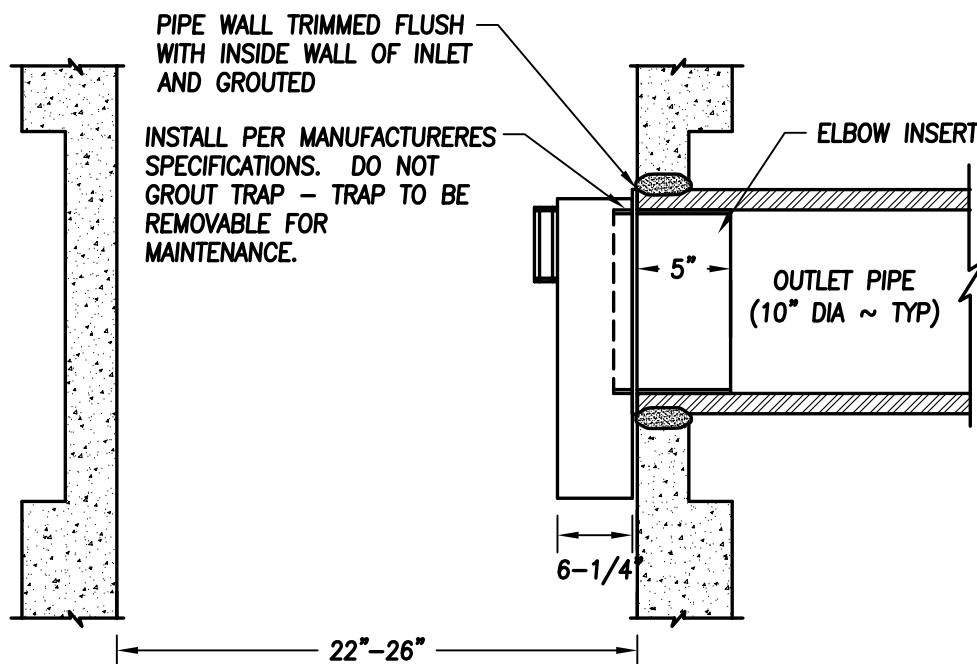
STANDARD CATCH BASIN TRAP NTS
