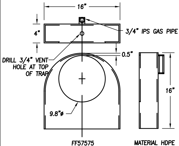
LOW PROFILE ELBOW NTS
