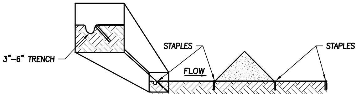
SILT DIKE UNIT – CUT SECTION
